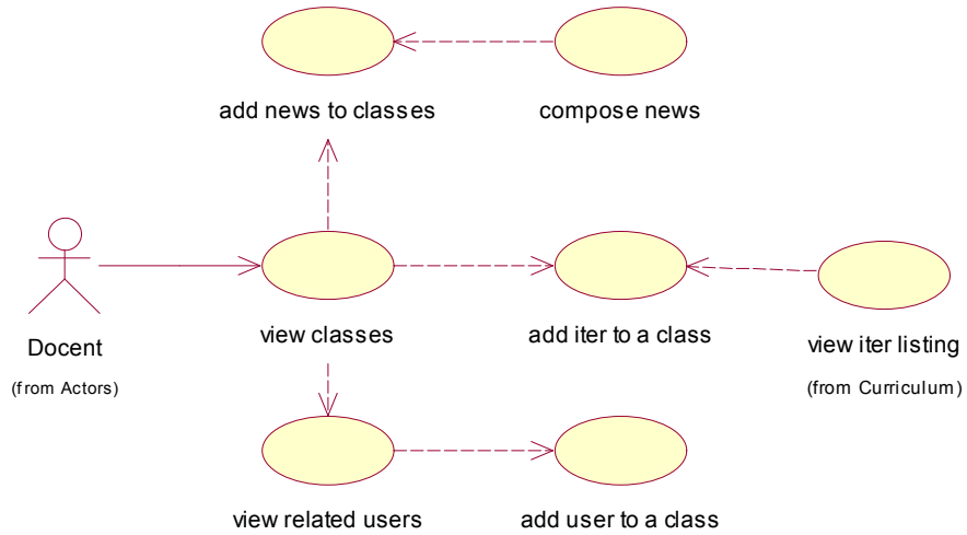
fig. 4 – main classes management use cases
