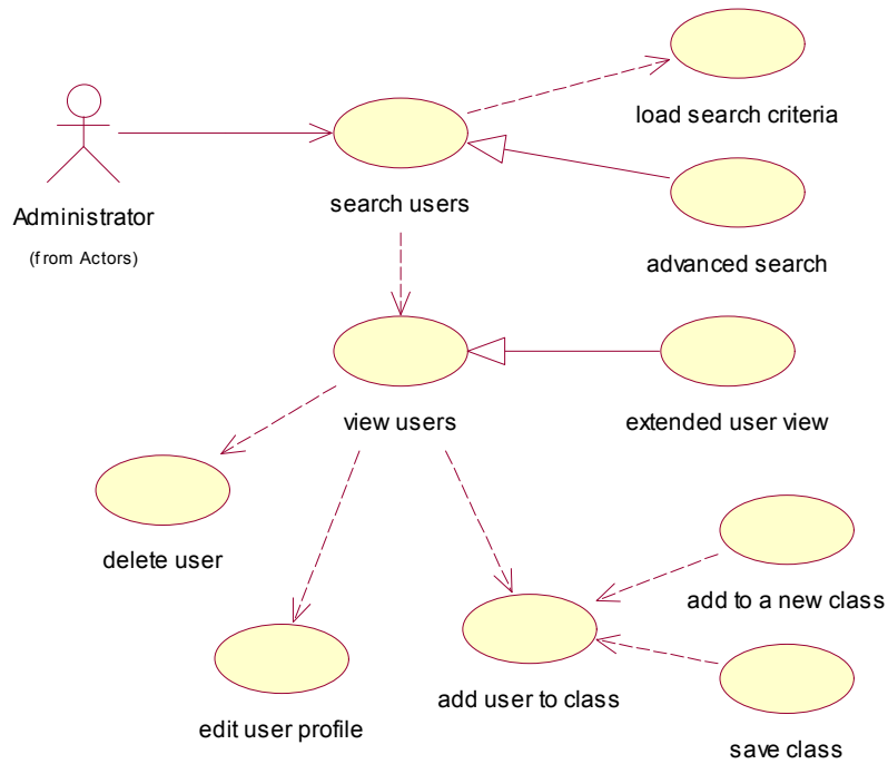
fig. 6 – main users and profiles management use cases
