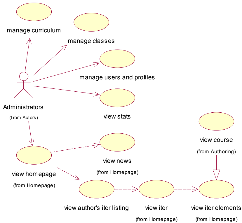
fig. 9 – main admin homepage use cases
