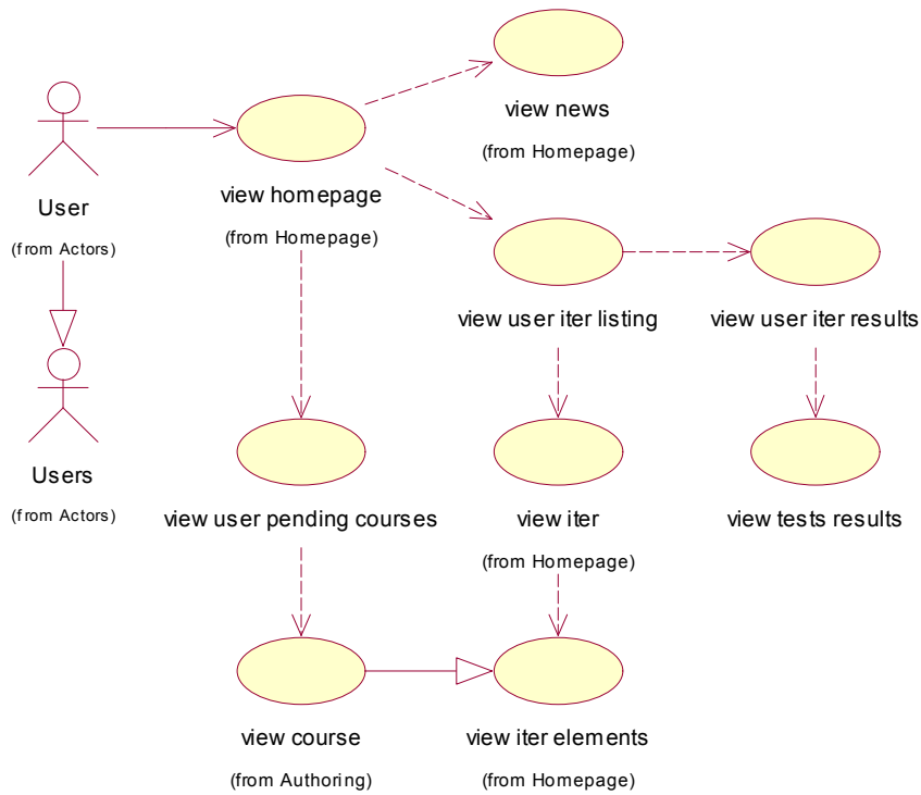
fig. 8 – main user homepage use cases
