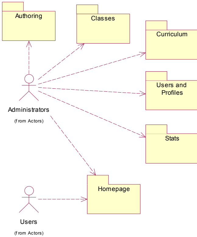
fig. 1 - main use cases packages
