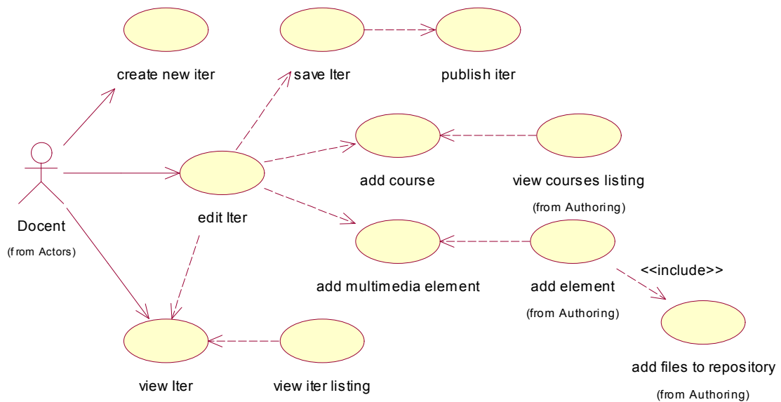
fig. 5 – main curriculum management use cases
